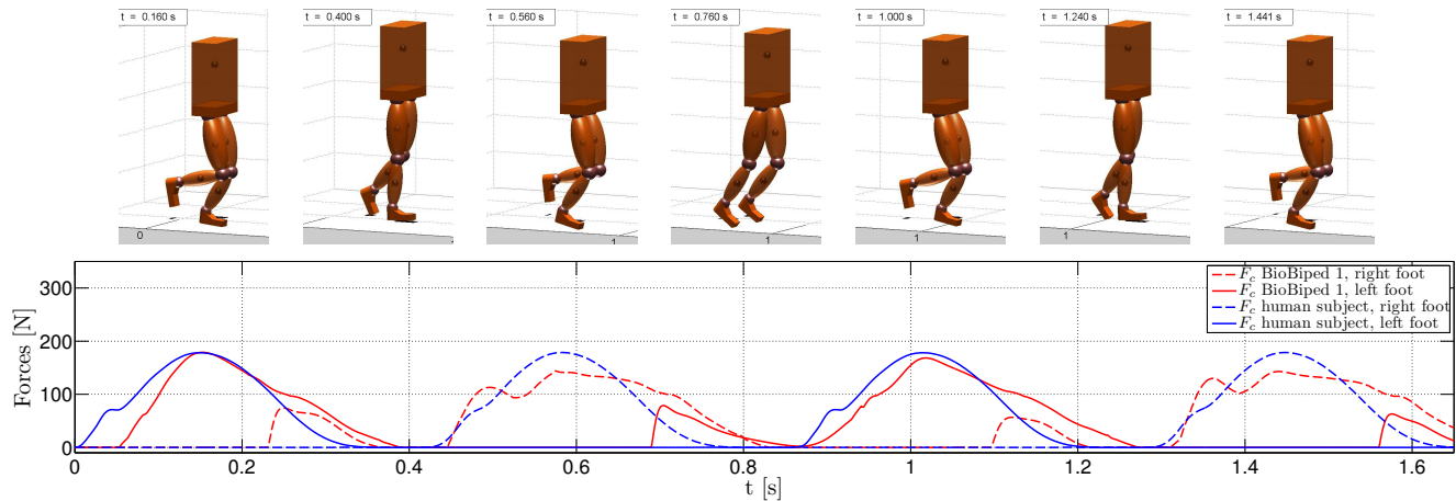
Fig. 11. Frames of the simulated BioBiped1 robot tracking a human-data based jogging motion with \sim 2\% . Simulated ground contact forces match the measured contact forces quite well.
